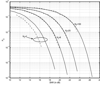
Fig. 3. (U) The bit error probability versus average signal-to-noise ratio for the proposed FSR-UWB system on an AWGN channel. Dashed lines correspond to simulation results, whereas solid lines correspond to the analytical results of (6).
