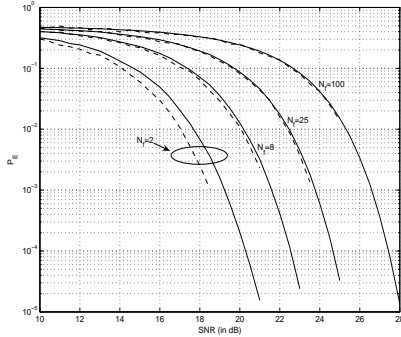
Fig. 4. (U) The bit error probability versus average signal-to-noise ratio for the standard TR-UWB system on an AWGN channel. Dashed lines correspond to simulation results, whereas solid lines correspond to the analytical results of (7).
