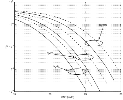
Fig. 5. (U) The bit error probability versus average signal-to-noise ratio for the TR-UWB system (dashed lines) and FSR-UWB system (solid lines) operating over a multipath fading channel. The system parameters are the same as those for Figure 3. Results are obtained by generating 10^5 random channels \underline{h} for each data point and using such to empirically estimate the expectations in (9) and (10).
