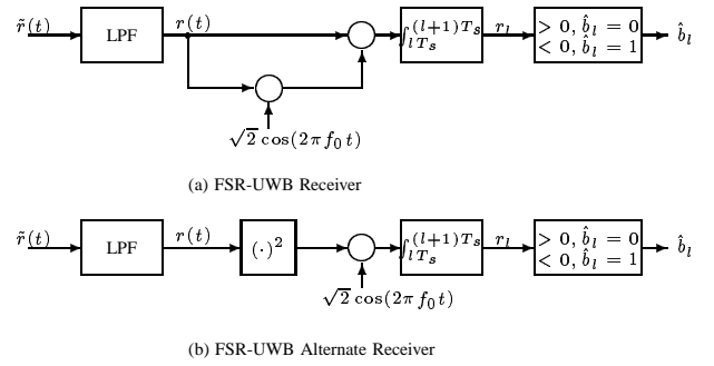
Fig. 2. (U) Receiver for the proposed FSR-UWB system. Note that the delay element in Figure 1 has been replaced by a mixer in (a). Since multiplication is commutative, the receiver in (a) can be drawn in the more convenient form given in (b).
