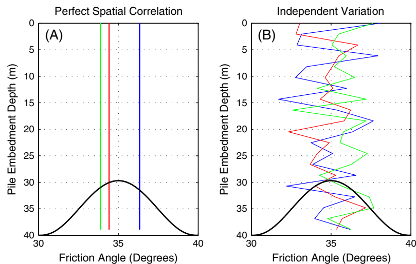
Figure 3. Sample realizations of random soil profiles in terms of friction angle. (a) Soil profile with perfect spatial correlation where a single random friction angle is defined for the entire depth of the pile. (b) Soil profile with the friction angle at each soil spring is independent of other soil springs. In both cases, the bold curve at the bottom defines the marginal beta distribution of the friction angle.
