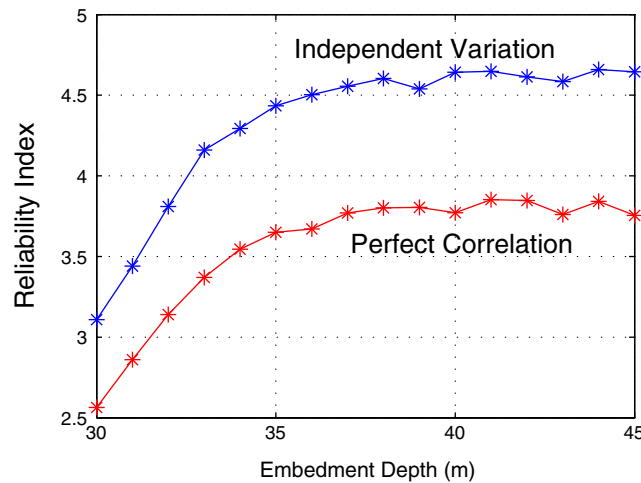
Figure 11. Reliability index as a function of embedment depth.
