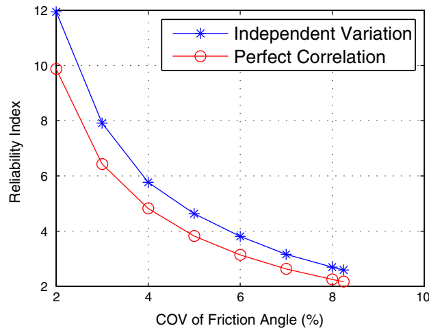
Figure 6. Reliability index versus COV of friction angle.
